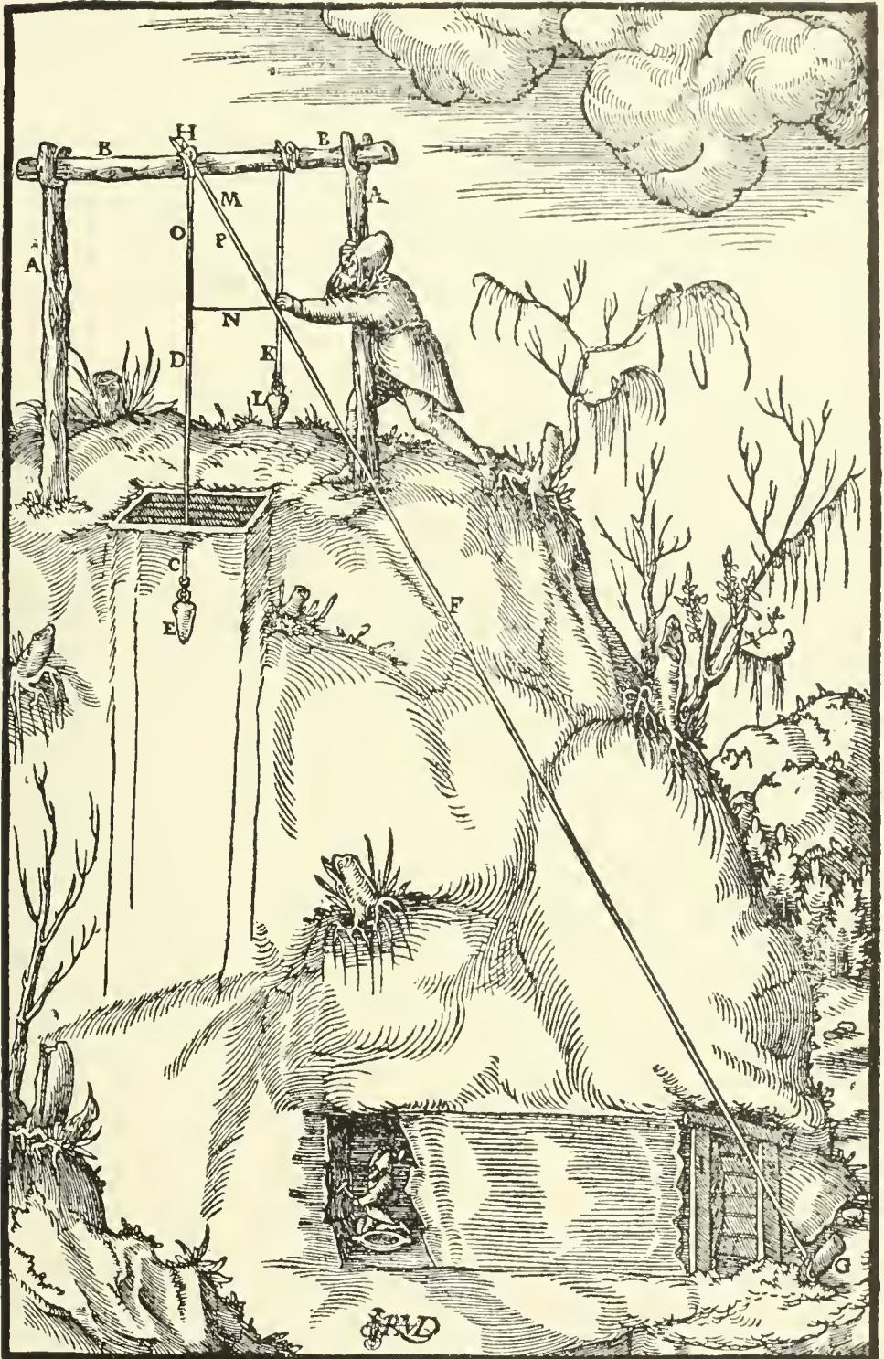
A—UPRIGHT FORKED POSTS. B—POLE OVER THE POSTS. C—SHAFT. D—FIRST CORD. E—WEIGHT OF FIRST CORD. F—SECOND CORD. G—SAME FIXED GROUND. H—HEAD OF FIRST CORD. I—MOUTH OF TUNNEL. K—THIRD CORD. L—WEIGHT OF THIRD CORD. M—FIRST SIDE MINOR TRIANGLE. N—SECOND SIDE MINOR TRIANGLE. O—THIRD SIDE MINOR TRIANGLE. P—THE MINOR TRIANGLE.
